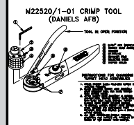
M22520/1-01 CRIMP TOOL (DANIELS AFB)
